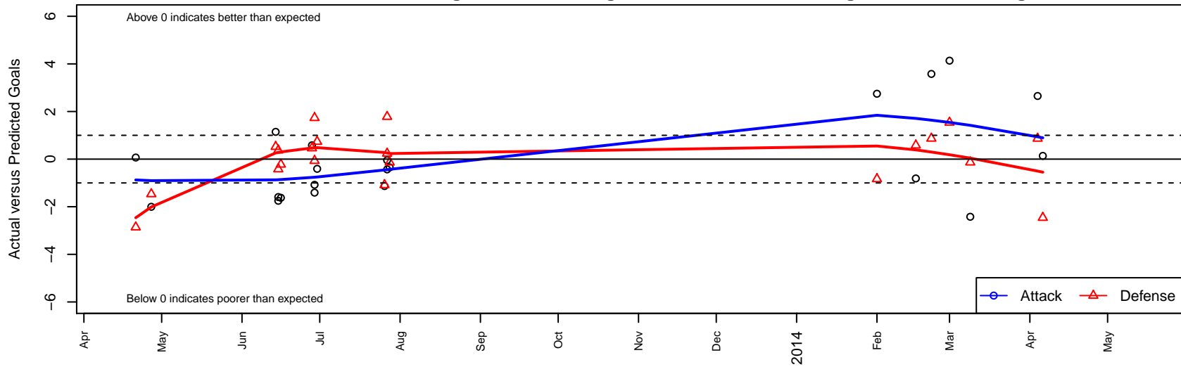
Crossfire Oregon Black B95 Dots are actual minus expected GF (blue circles) and GA (red triangles). Blue line is smoothed change in attack strength. Red is smoothed change in defense strength.
